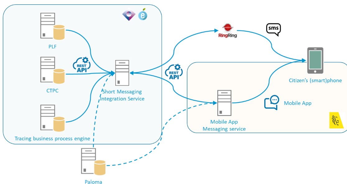
Figure 1 High-Level Architecture
